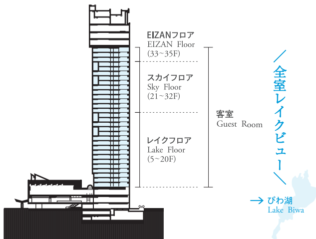
Hotel Plan Side View
